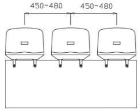
Simple mount
