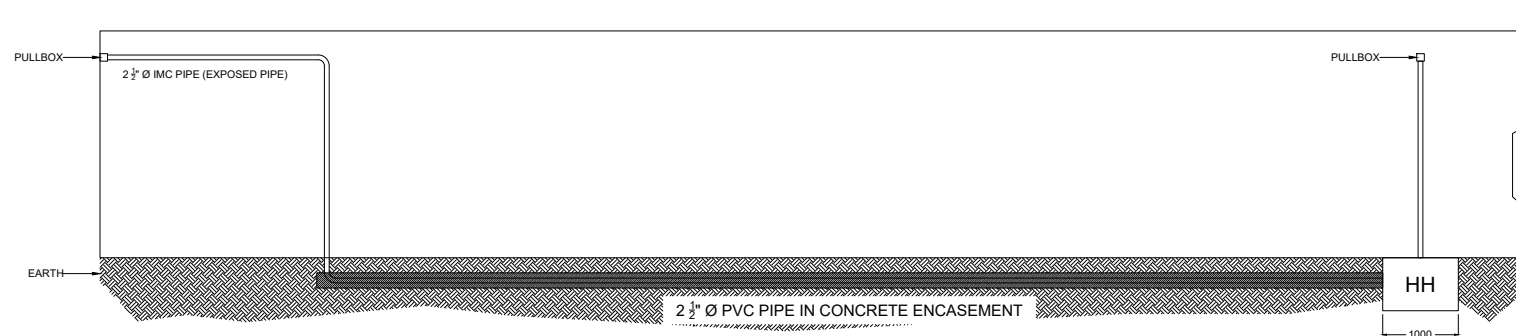
SECTION B-B DETAIL
