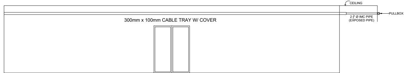
SECTION A-A DETAIL
